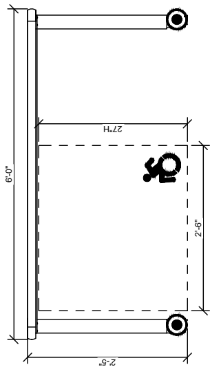
FRONT ELEVATION
