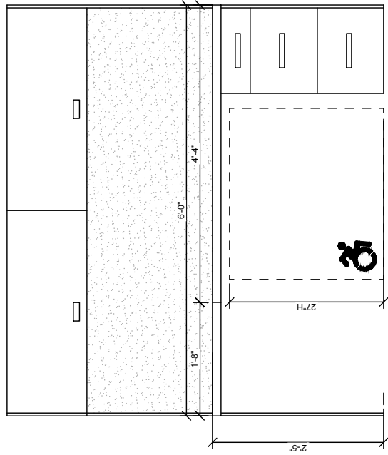
FRONT ELEVATION
