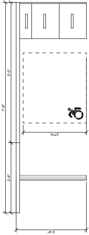
FRONT ELEVATION
