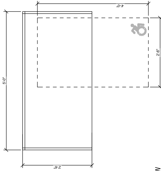
PLAN VIEW D04
