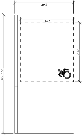
FRONT ELEVATION
