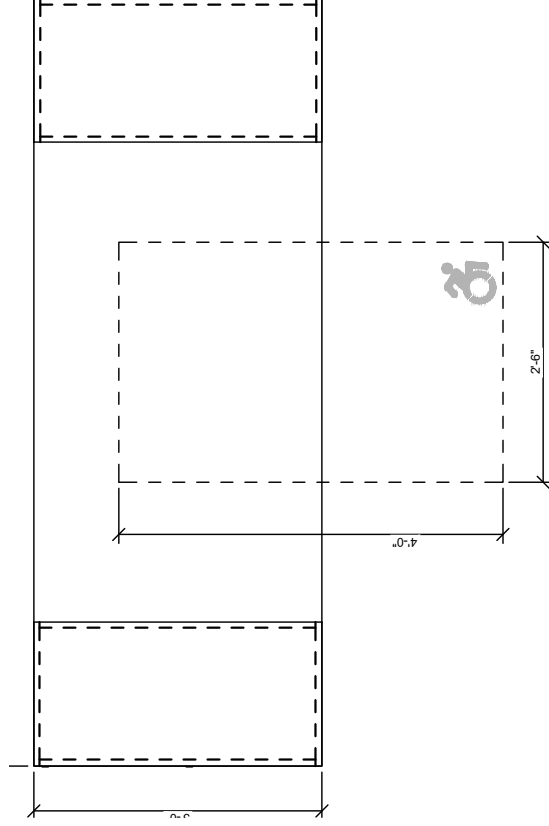
PLAN VIEW
